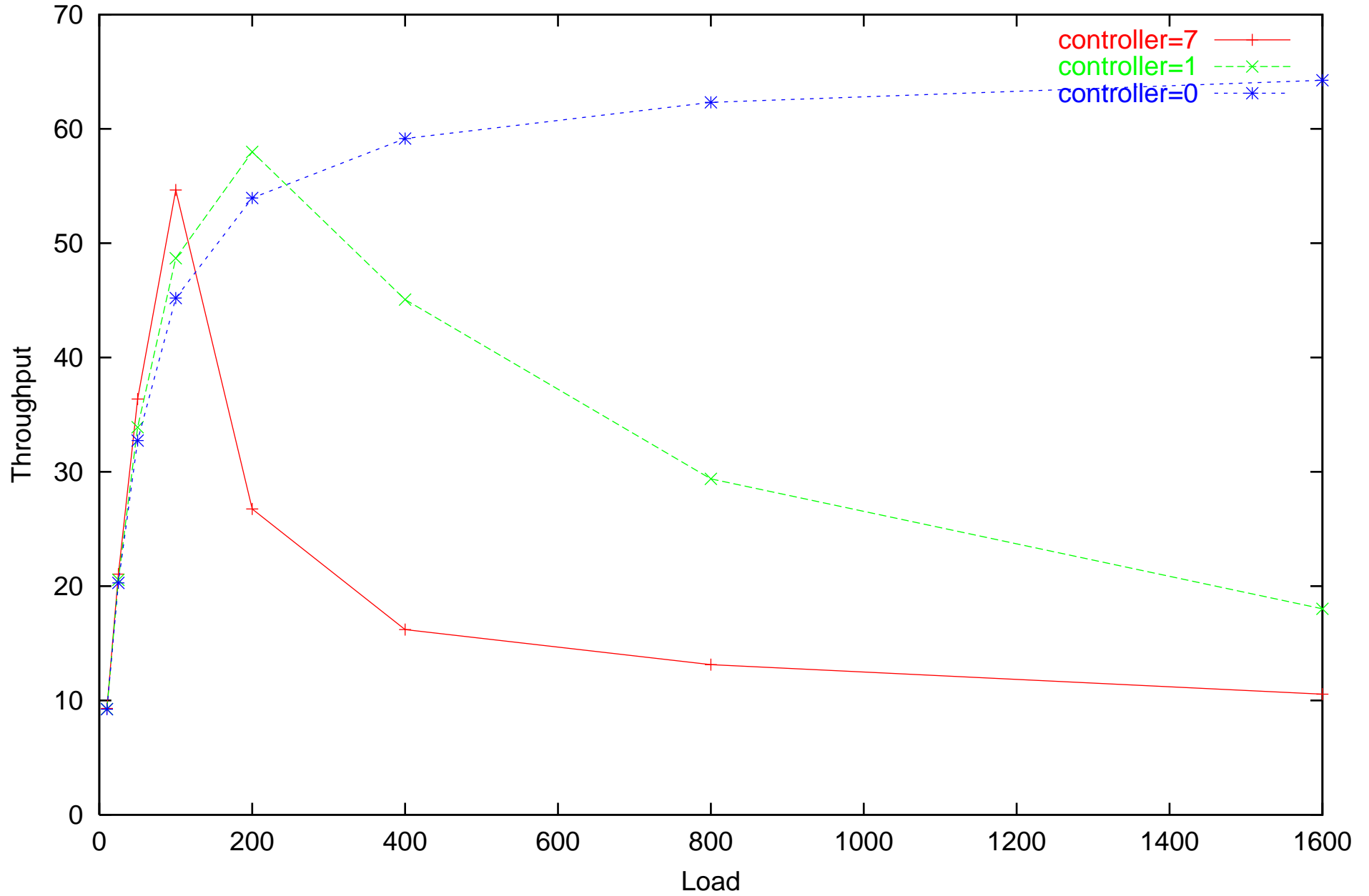
Load-dependent throughput for low priority disk
