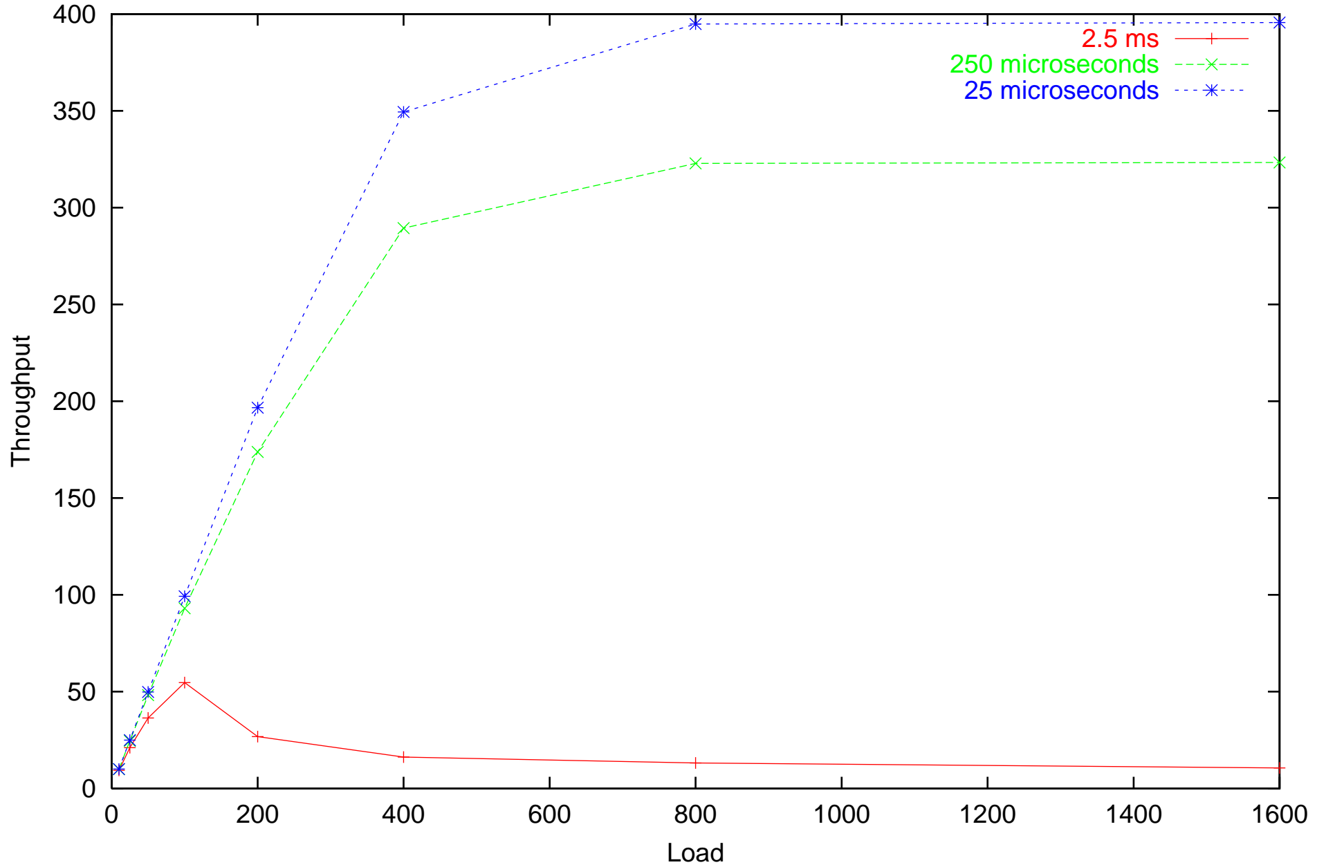
Low priority disk throughput for different values of bus delay
