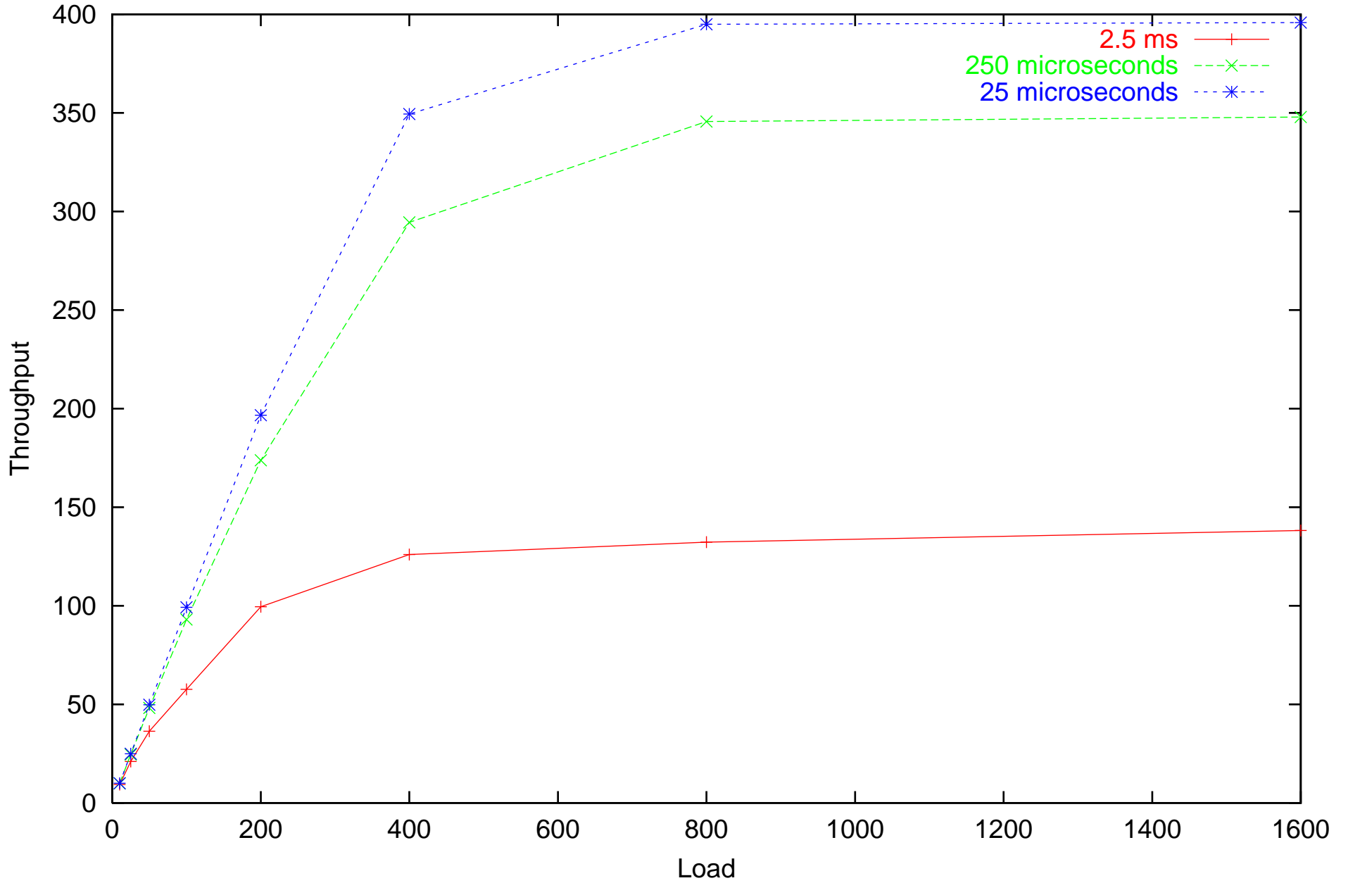
High priority disk throughput for different values of bus delay
